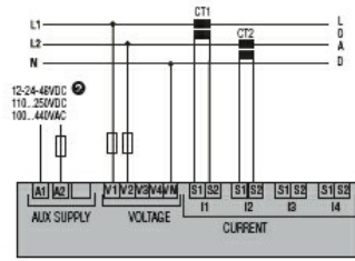
Two-phase
