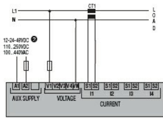
Single-phase
