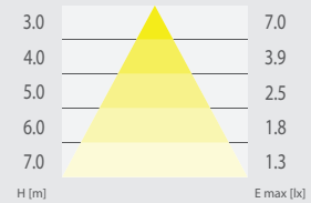
Starlet Round LED SC 350
