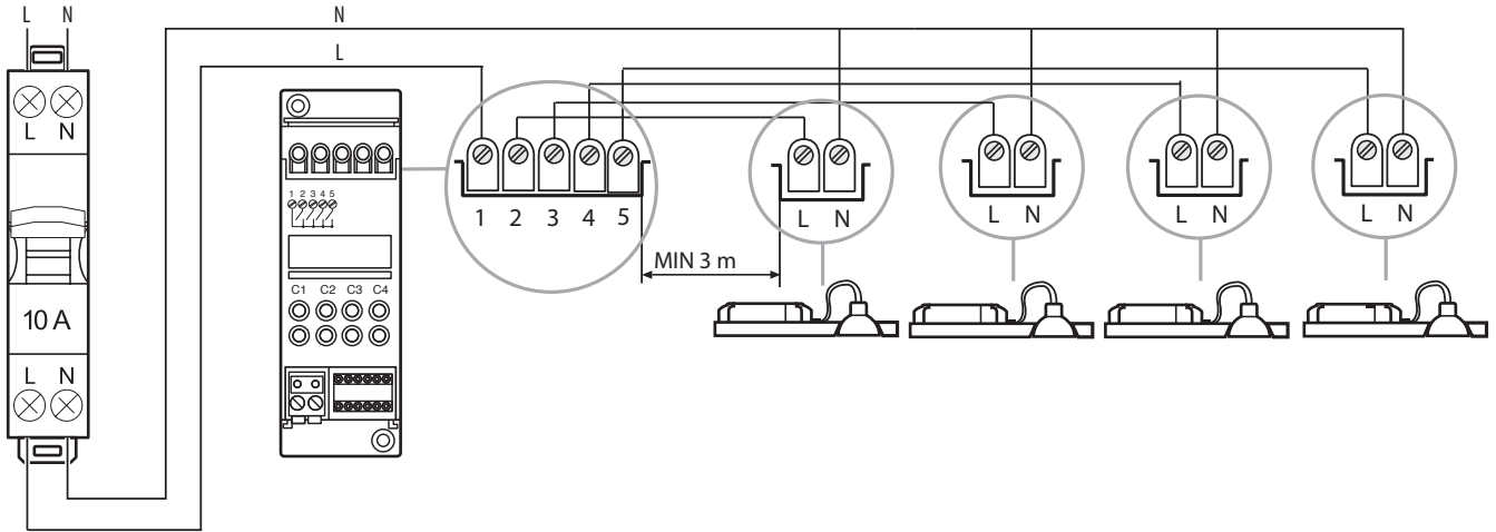
Diagram for connecting light devices
