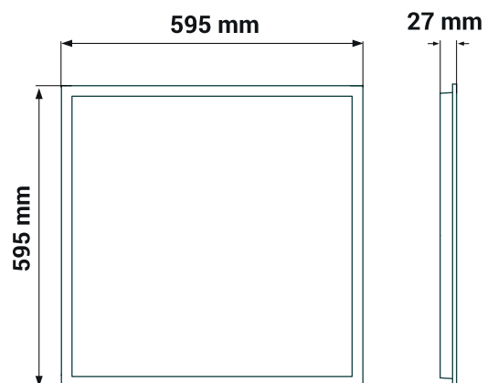
ORO BACKLIT LED 36W 60X60 NW CCT
