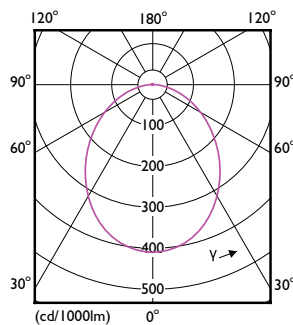
Light Distribution Diagram - PILA LED 500lm GU10 CW 120D ND 1CT/10
