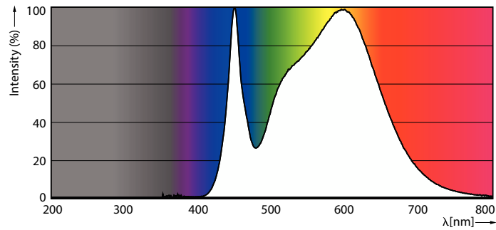
Spectral Power Distribution Colour - PILA LED 500lm GU10 CW 120D ND 1CT/10
