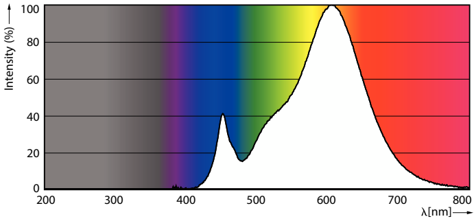
Spectral Power Distribution Colour - PILA LED 100W A60 E27 WW FR ND 1CT/6
