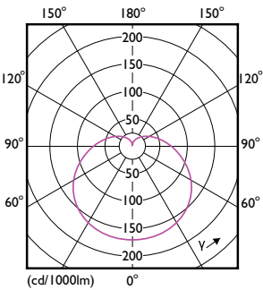
Light Distribution Diagram - PILA LED 100W A60 E27 WW FR ND 1CT/6
