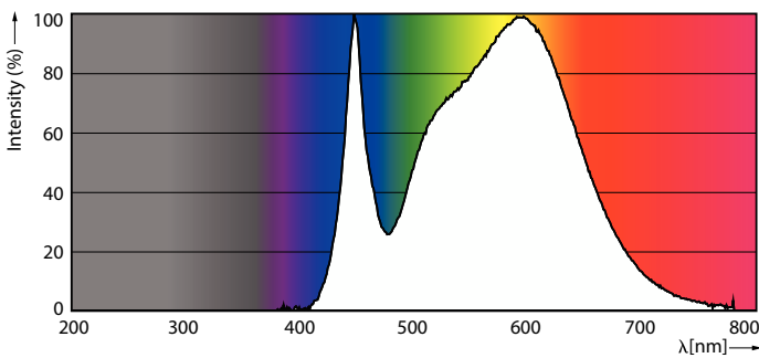
Spectral Power Distribution Colour - CorePro lustre ND 2.8-25W E14 840 P45 FR
