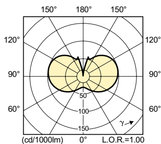
Light Distribution Diagram - MASTER CityWh CDO-ET Plus 50W/828 E27
