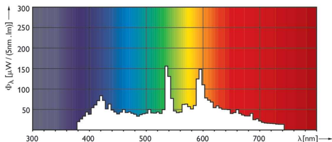
Spectral Power Distribution Colour - MASTERC CDM-TC 35W/842 G8.5 ICT/12
