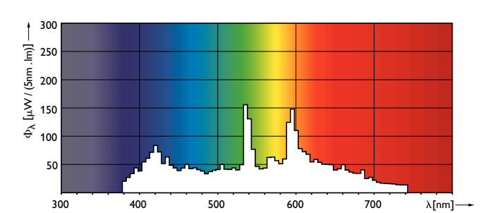
Spectral Power Distribution Colour - MASTERC CDM-T 35W/842 G12 1CT/12
