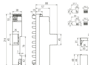
Dimension drawing DSH ZP 2 SG TNS 255
