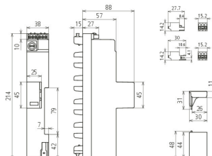
Dimension drawing DSH ZP B2 SG TNS 255
