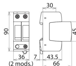
Dimension drawing DG MU SP 240 3W+G
