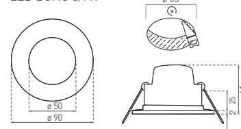
LED BONO 5/7W
