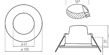
LED BONO 8W
