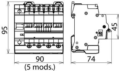
Dimension drawing POP 4 255 C25
