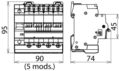
Dimension drawing POP 4 255 C32
