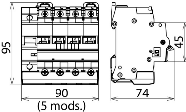
Dimension drawing POP 4 255 C63
