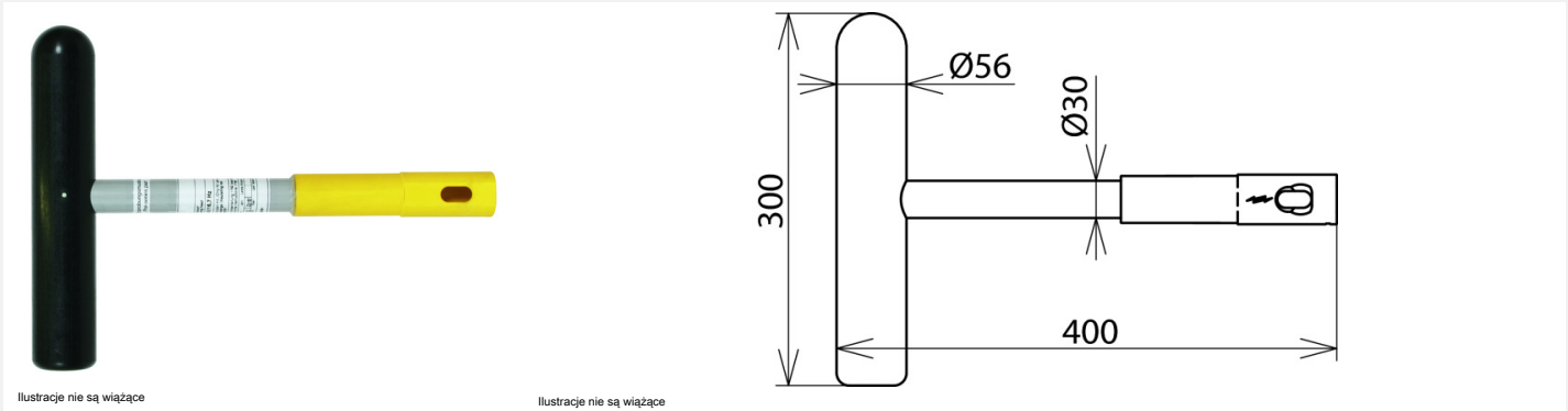
Operating head (hammer) with plug-in coupling
