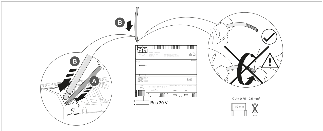
Fig. 10: Connecting the device
