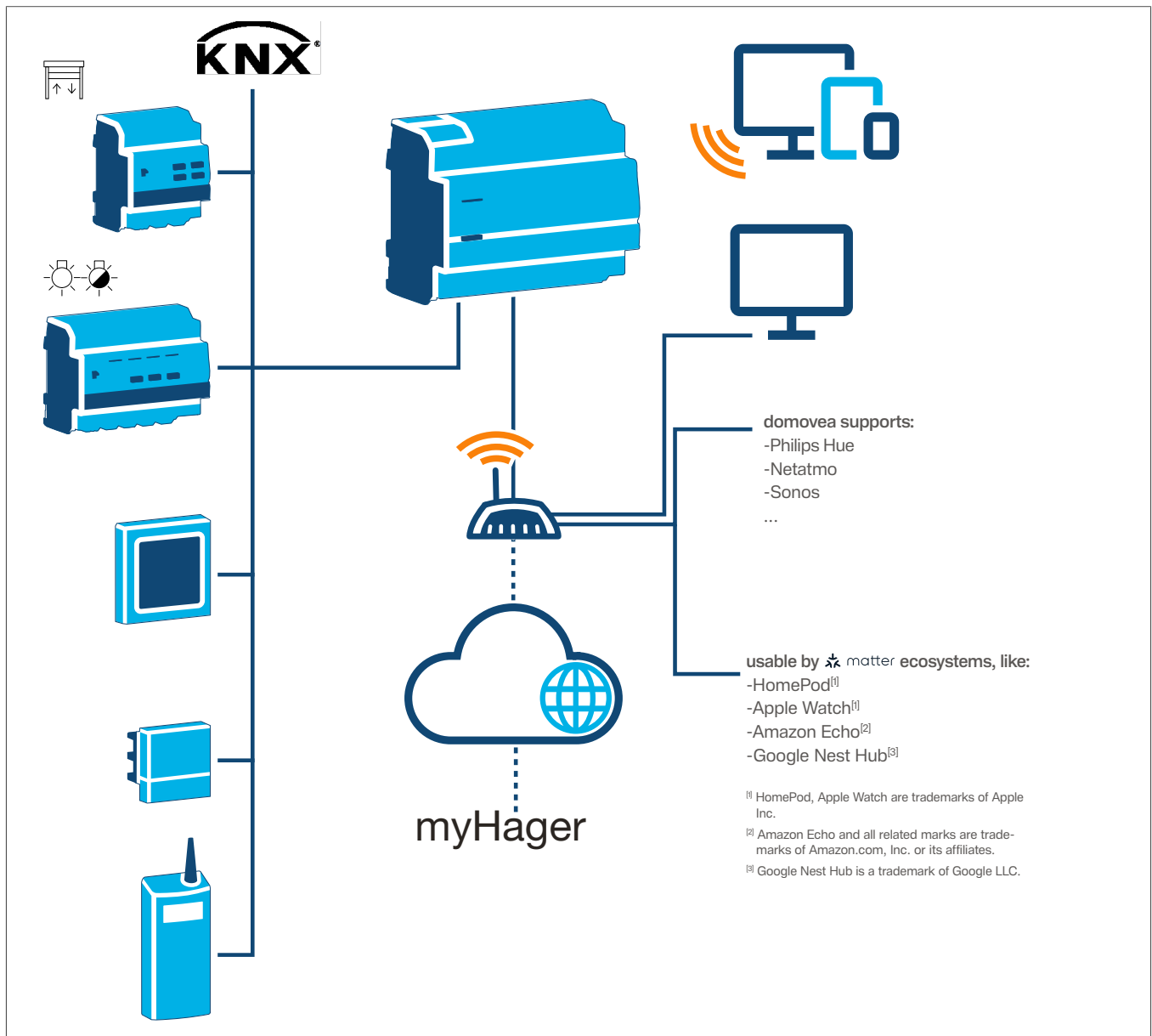
Fig. 7: System overview
