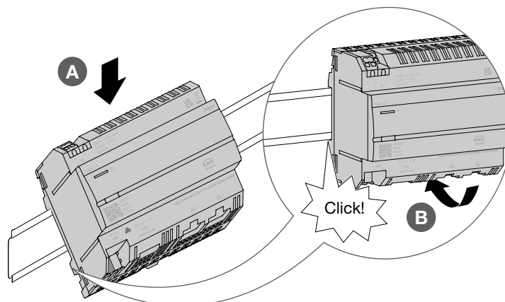
Fig. 9: Mounting the device on the DIN rail
