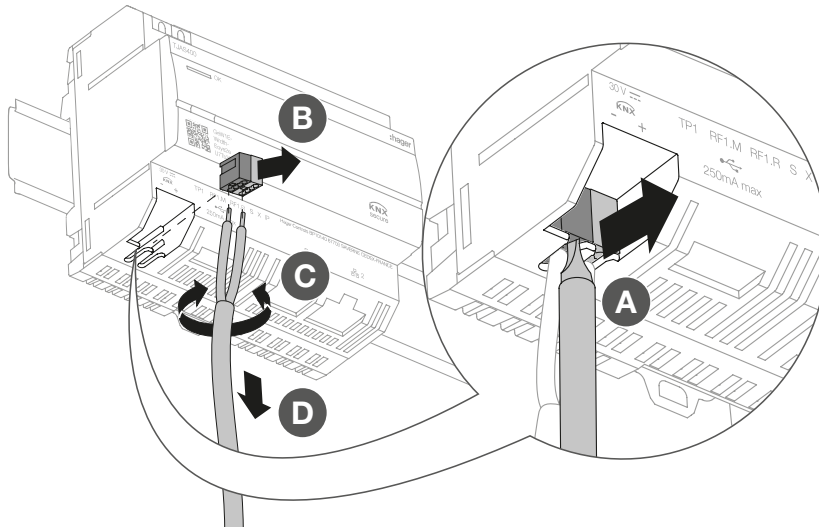
Fig. 15: Removing the bus connection terminal
