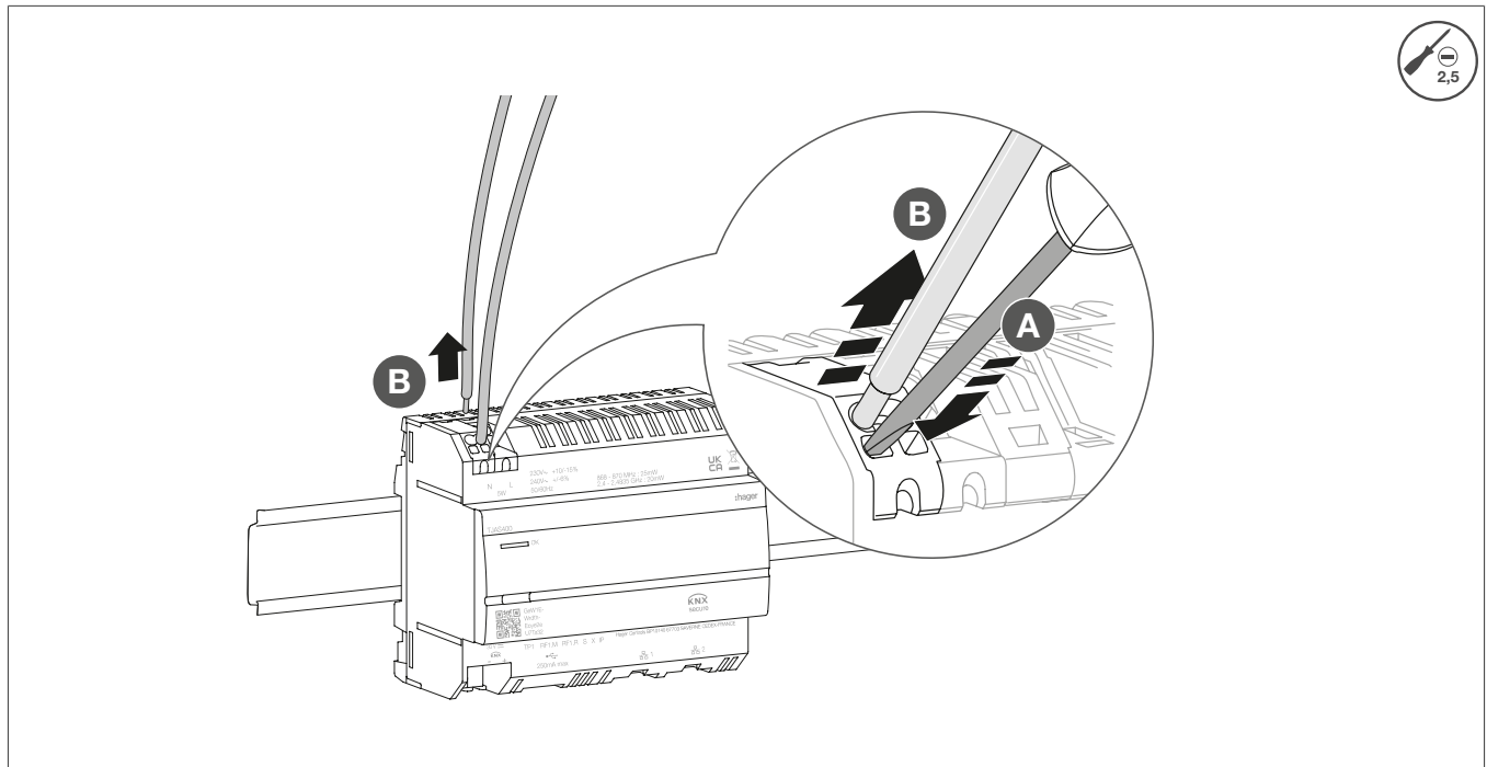
Fig. 14: Disconnecting the connection cables
