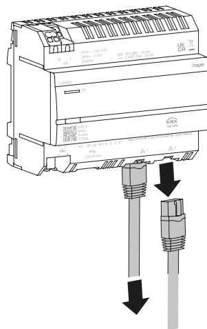
Fig. 16: Disconnecting the network cable
