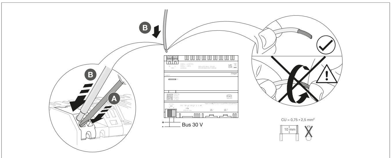
Fig. 11: Connecting the device
