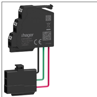
HWY950HSA
