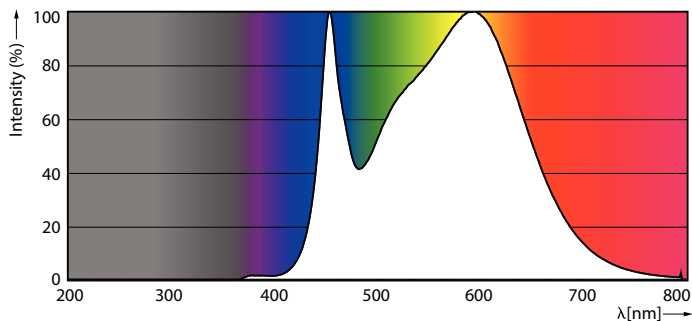
Spectral Power Distribution Colour - Corepro LEDspot 2.7-25W GU10 840
