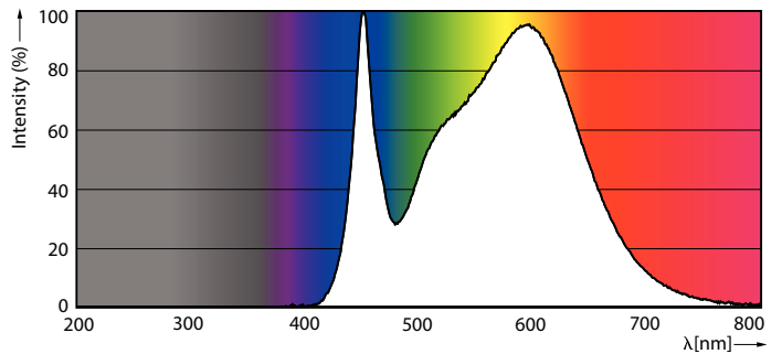
Spectral Power Distribution Colour - LEDbulb ND 4.9-40W A60 E27 840 1CT
