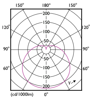
Light Distribution Diagram - LEDbulb ND 4.9-40W A60 E27 840 1CT
