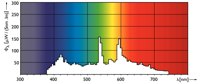
Spectral Power Distribution Colour - MASTERC CDM-T 35W/842 G12 1CT/12
