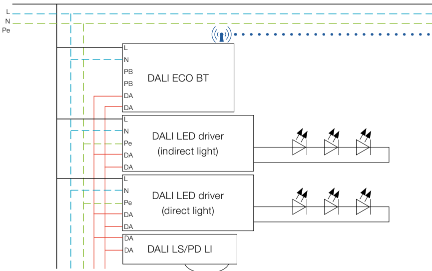
a) Wiring diagram of floor-standing luminaires shown in the Swarm zone
