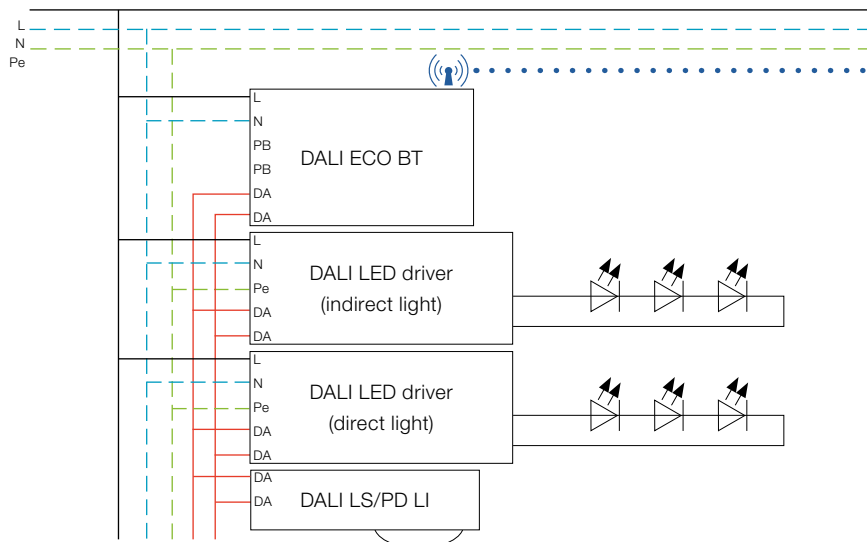
c) Wiring diagram of floor-standing luminaires shown in zones 1-4
