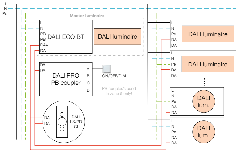
d) Wiring diagram of zone 5 with standard DALI luminaires
