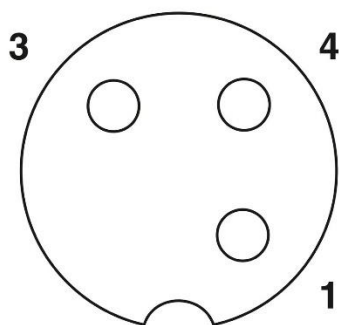
Pin assignment M12-jack, 3-pol, A-coding
