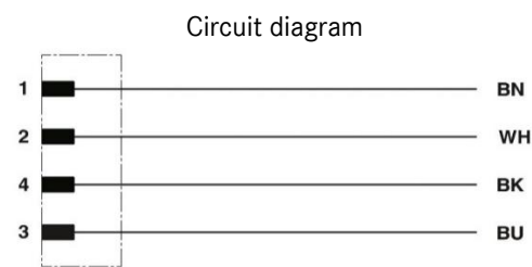
Pin assignment M12-plug
