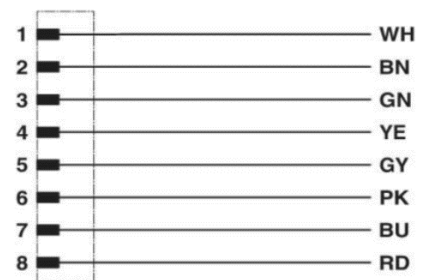
Pin assignment from M12-plug
