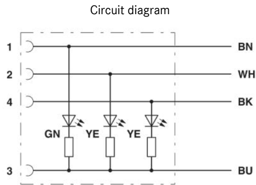
Pin assignment between M12-plug and M12-jack, with LED
