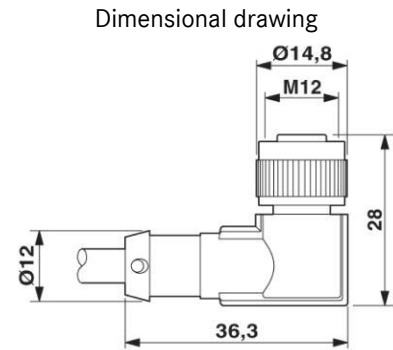
Jack M12 x 1, angled, with LED
