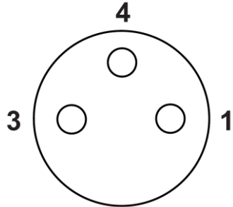
Pin assignment M8-jack, 3-pol, A-coding
