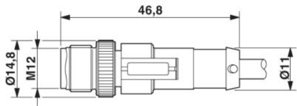
Dimensional drawing
