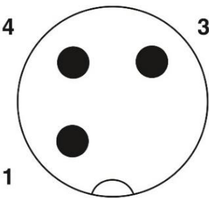
Pin assignment M12-plug, 3-pol, A-coding
