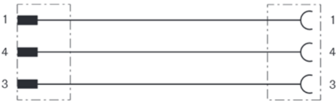
Pin assignment between M12-plug and M12-jack
