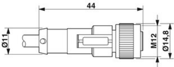
Jack M12 x 1, straight
