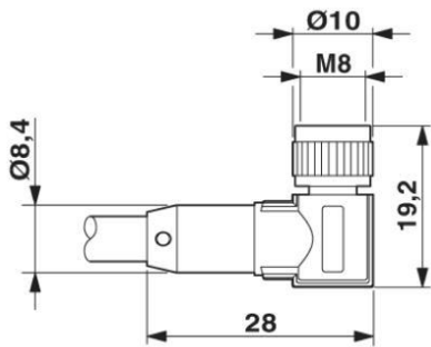
Jack M8 x 1, angled, with LED
