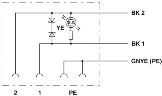
Pin assignment of valve connector
