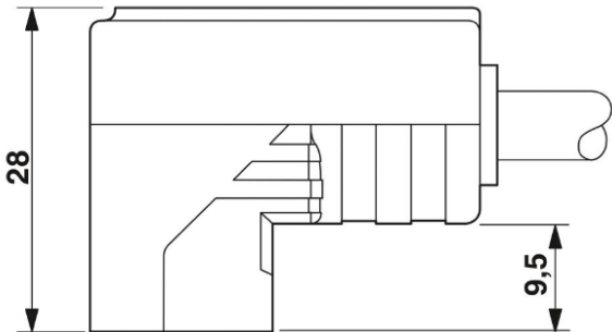
Valve connector, type C, side view
