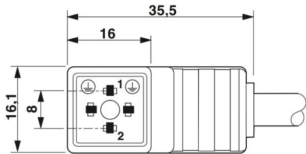
Valve connector, type CI
