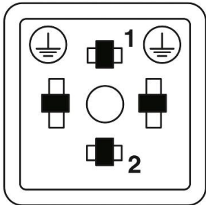
Valve connector, type CI
