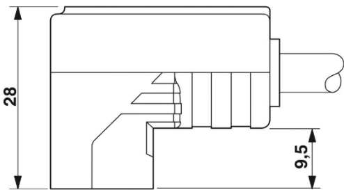
Valve connector, type CI, side view
