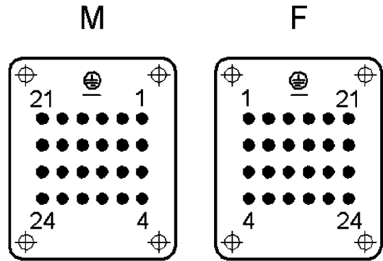
Pin diagram, cable connection side
