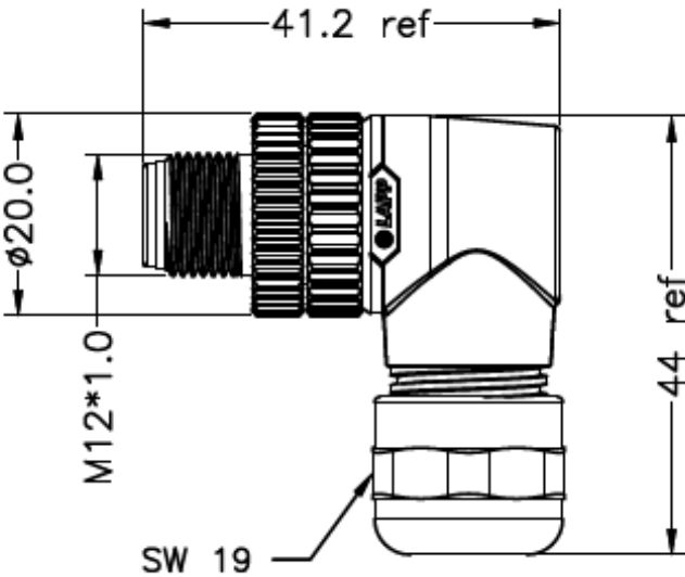
Technical drawing
