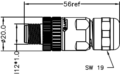
Technical drawing
