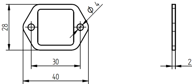
Flat Gasket, H-A 3 (10607100)
