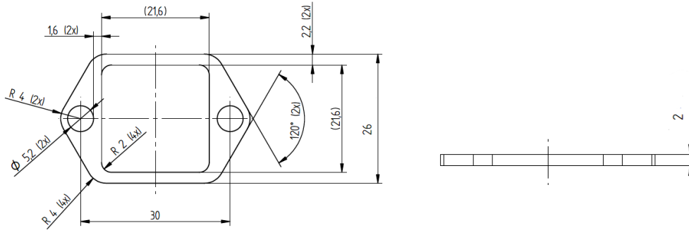
Flat Gasket, H-A 3 (38116823)
