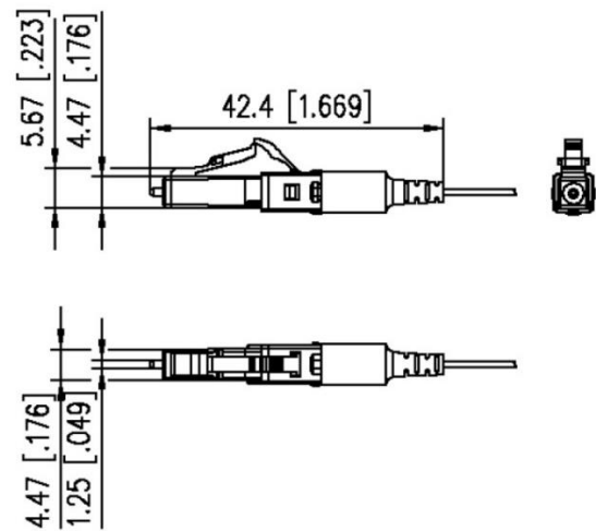
Dimensional drawing
