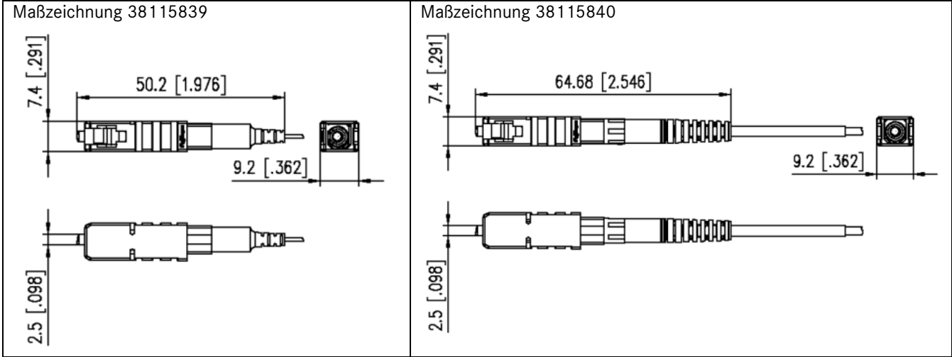
Dimensional drawing
