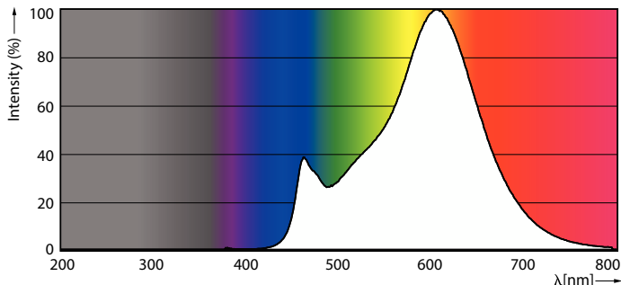
Spectral Power Distribution Colour - LED cła 120W G120 E27 WW FR ND RFSRT4
