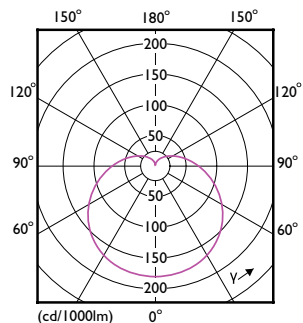
Light Distribution Diagram - LEDbulb ND 10-75W A60 E27 840 1CT
