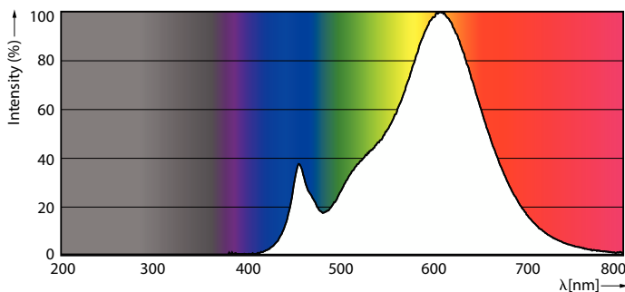
Spectral Power Distribution Colour - LEDbulb ND 4.9-40W A60 E27 827 1CT
