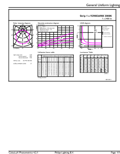
General uniform lighting - MAS LEDstrip 21.3W930 2400LM/M 5M
