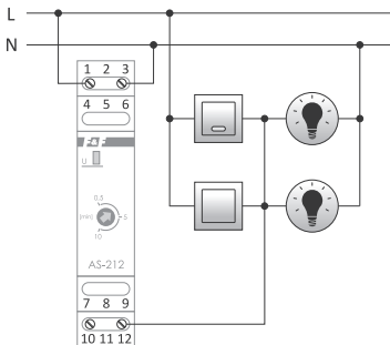
3-wire installation
