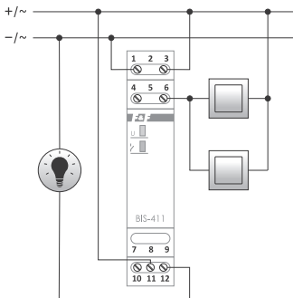
Connection with control pulse +
