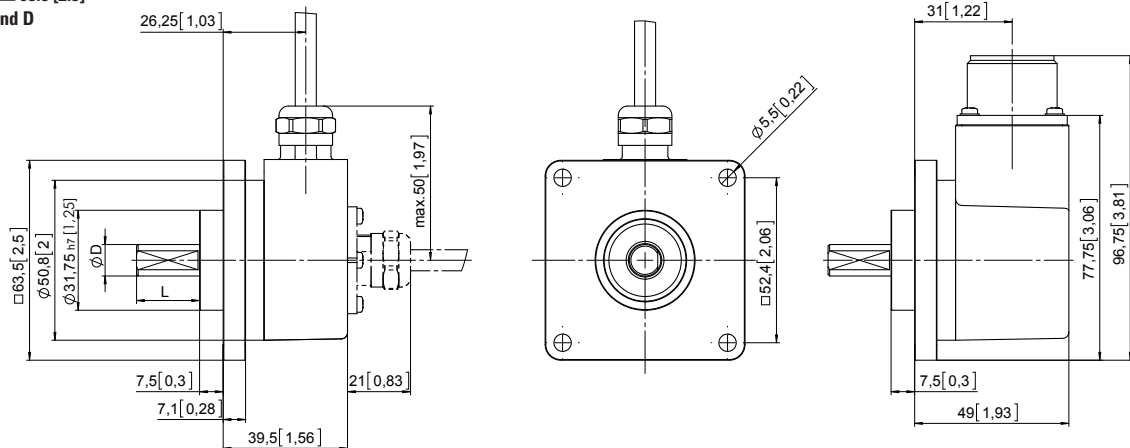
MIL-connector version
