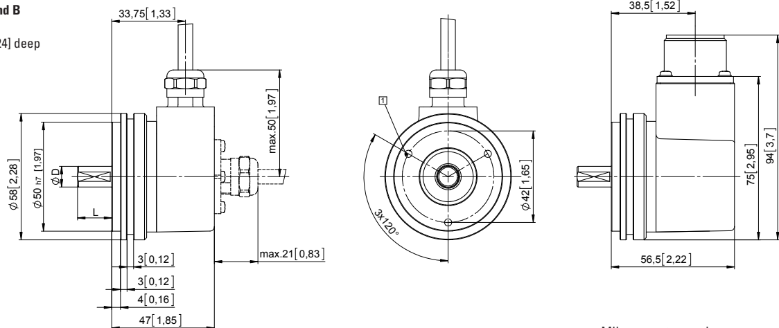
MIL-connector version
