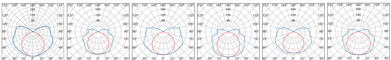
DUST EVG PC 1 ×18W
